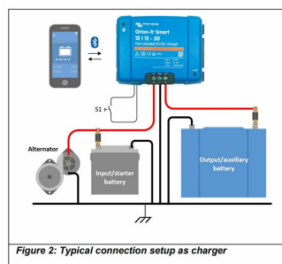
Figure 2: Typical connection setup as charger
